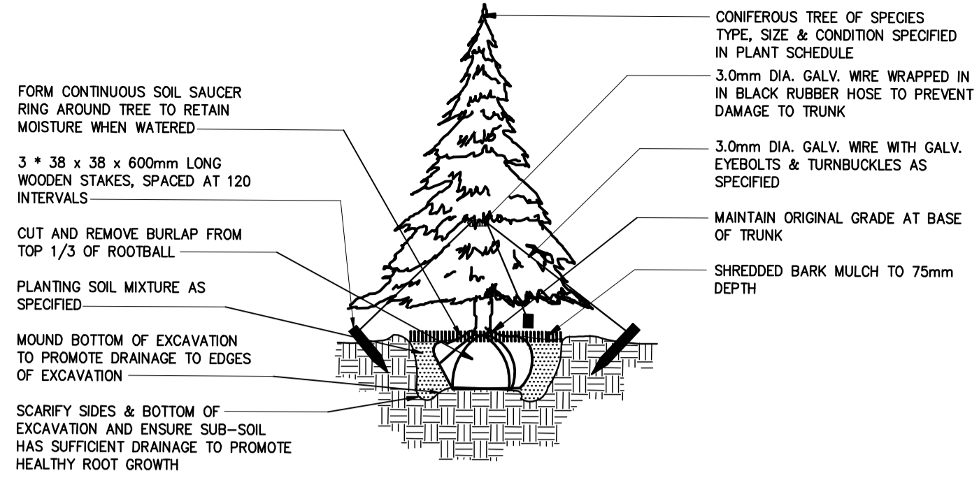
CONIFEROUS TREE NTS
